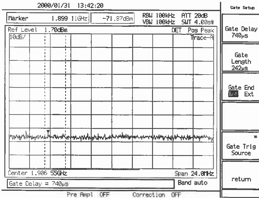
Example of Carrier-Off Leakage Power P (L) Measurement
