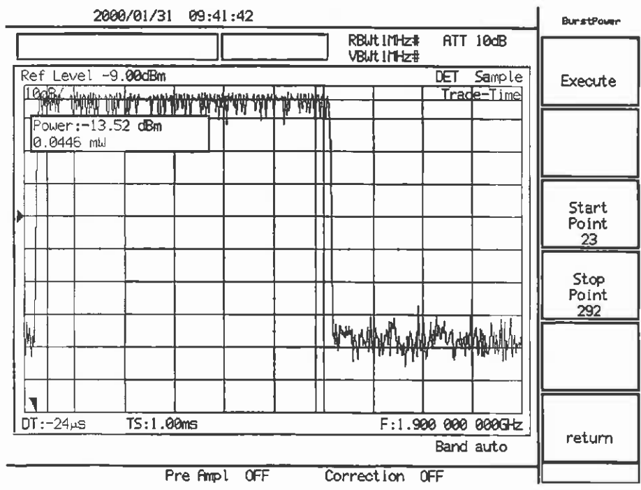
Power Measurement (Time Domain) Example 1
