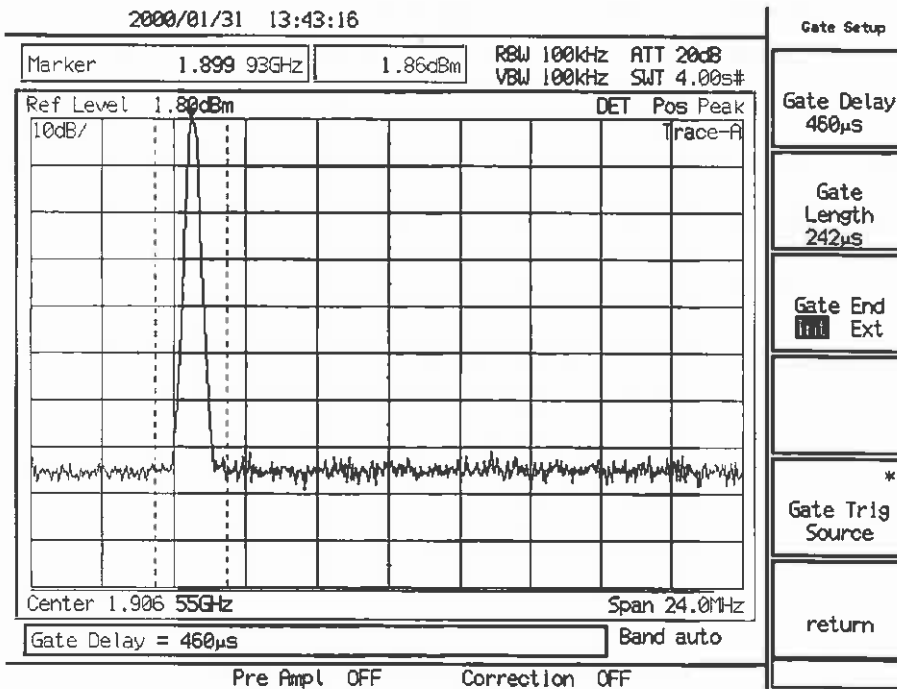
Example of Carrier-On Leakage Power P (O) Measurement
